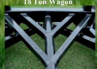
Double Webbing On G36T 18 Ton Wagon
